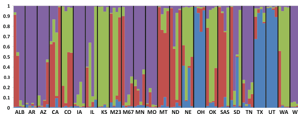
Fig. 2 STRUCTURE plot of 96 wild H. annuus individuals with K = 4 clusters. Blue, cluster 1; red, cluster 2; green, cluster 3; purple, cluster 4. The y-axis shows the proportion membership into the various clusters. Each colored vertical bar represents a single wild individual and the 4 individuals from each of the 24 sampled populations are grouped together. Vertical black bars have been
