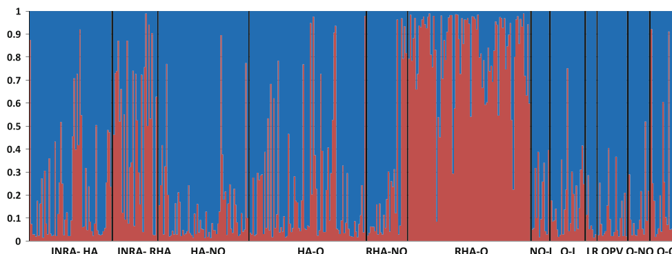
Fig. 3 STRUCTURE plot of the 433 cultivated sunflower accessions with K = 2 clusters. Blue, cluster 1; red, cluster 2. The y-axis shows the proportion membership into the various clusters. This analysis was based on a single individual per accession using genotypic data from 34 EST-SSRs (see “Methods” for details). The vertical black bars have been included as visual separators between the named
